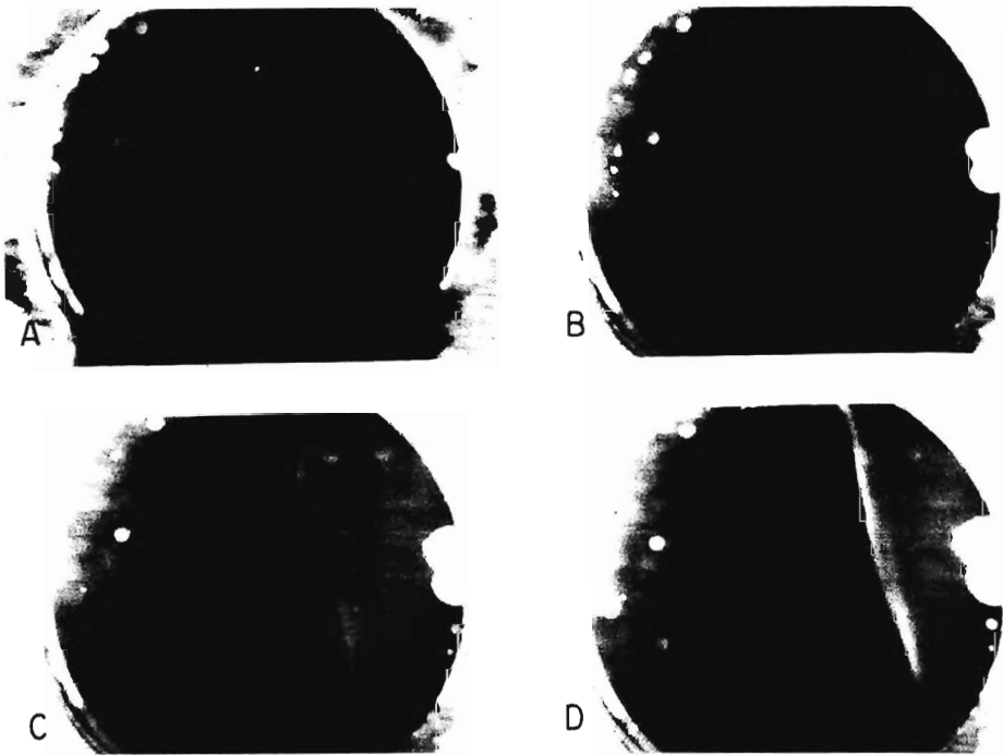
Fig. 1. Effect of passing current through a dilute solution of acid-soluble collagen. A t = 0 ; B 1 min; C 3 min; D 8 min. At 10 volts maximum current 65 \mu a . Chamber diameter, 0.5 inch. Electrodes along the horizontal, cathode at right. Exposure time 8 sec
